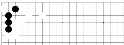
problem 271
