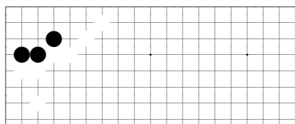
problem 331
