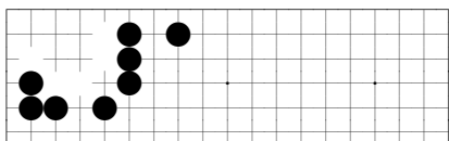
problem 366
