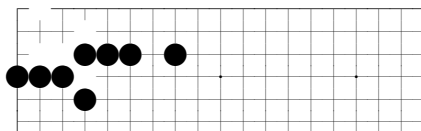
problem 127
