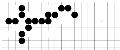
problem 172
