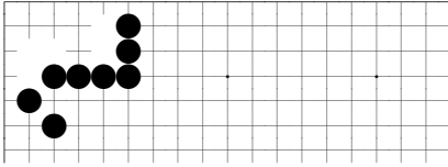
problem 418
