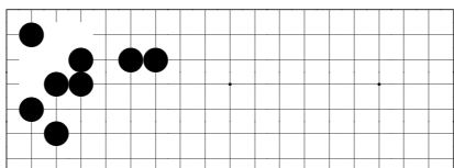
problem 146
