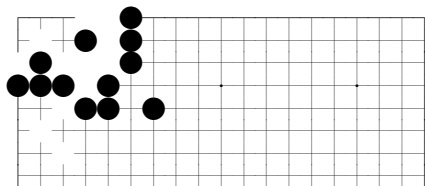
problem 479
