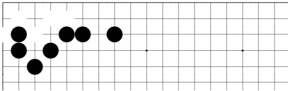
problem 57
