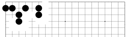
problem 54
