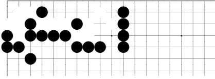
problem 78
