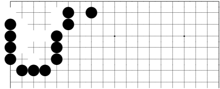
problem 634
