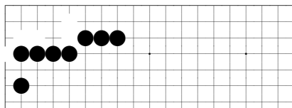
problem 402
