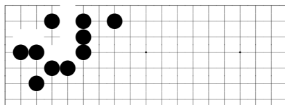
problem 412
