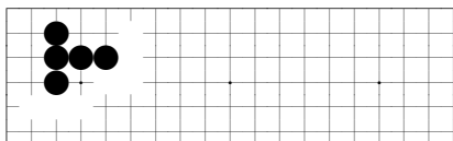
problem 432
