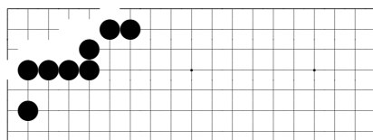
problem 392
