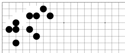
problem 192
