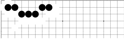
problem 316
