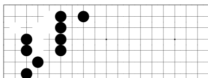
problem 300
