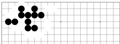
problem 168
