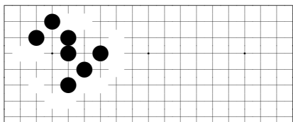
problem 198
