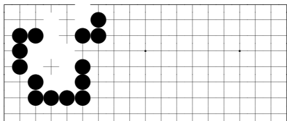
problem 767
