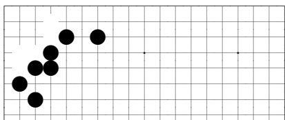
problem 561
