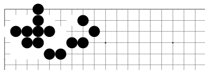
problem 76
