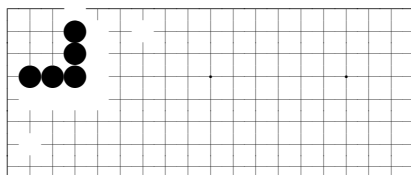
problem 574
