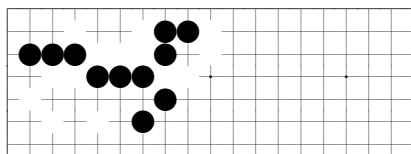
problem 439
