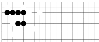
problem 532
