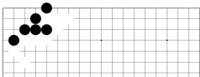
problem 199
