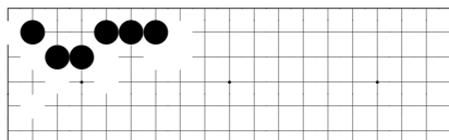
problem 647
