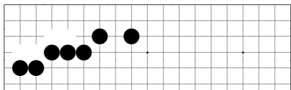
problem 339
