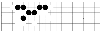
problem 645
