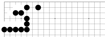
problem 97
