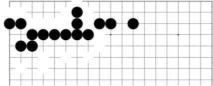
problem 229
