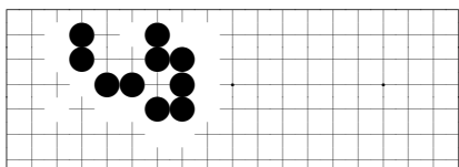
problem 722
